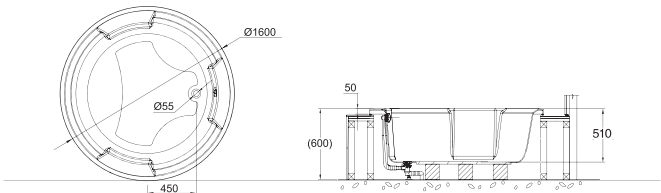
PARISIAN TB25615DW-4-1 Recessed Bathtub Ø 1600x510mm
