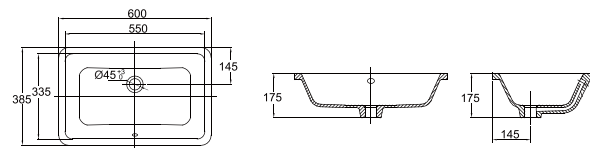
C22171W Glacier Undercounter Basin 600x385x175mm
