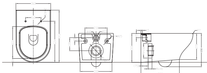
C01017XWJ C01017XW Real Wall Hung Toilet 540x360x350mm
