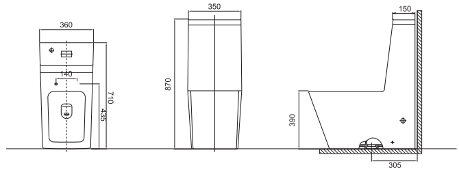
C02001W-3 Glacier One-piece Toilet 710X360X870mm
