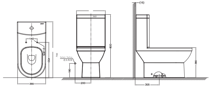
C2193XW-3 New Moon One Piece 700x360x800mm
