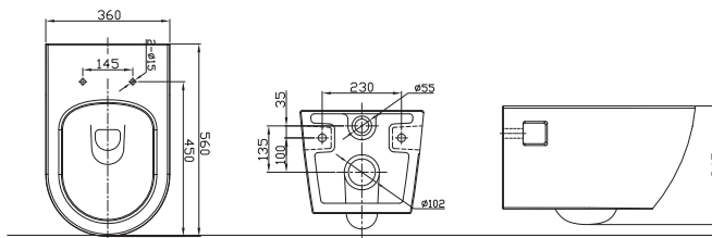
C2190UW Gina Wall Hung Toilet 560x360x345mm
