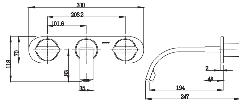
DM-2-002 Three hole Concealed Basin Mixer Wall Mounted Trim Kit (To be used with CB-003)
