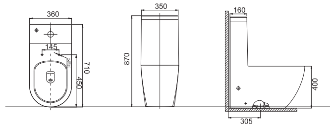
C02005W-3 Gina One-piece Toilet 710X360X870mm
