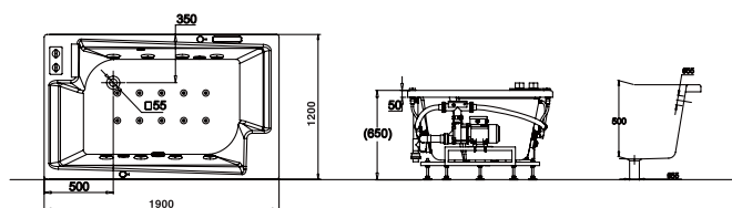
SOHO-1 TB25904DW-4-2 Recessed Massage Bathtub 1900x1200x650mm
