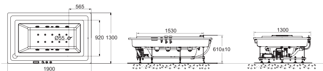
INFINITY TB25903DW-4-1 Recessed Massage Bathtub 1900x1300x610mm
