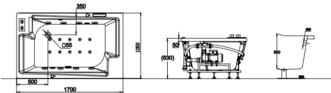
SOHO-2 TB25704DW-4-1 Recessed Massage Bathtub 1700x1050x630mm
