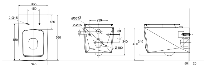
C2196W Diamond Wall Hung Toilet 560x365x340mm
